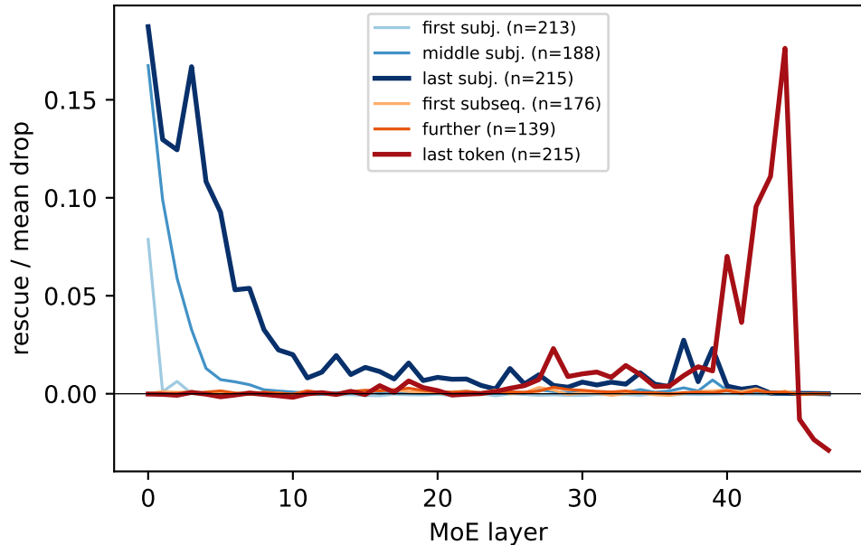
Qwen3-30B-A3B-Base: single-layer MoE patch at each token group
