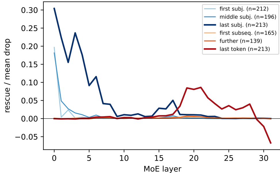
Mixtral-8x7B, BOS: single-layer MoE patch at each token group
