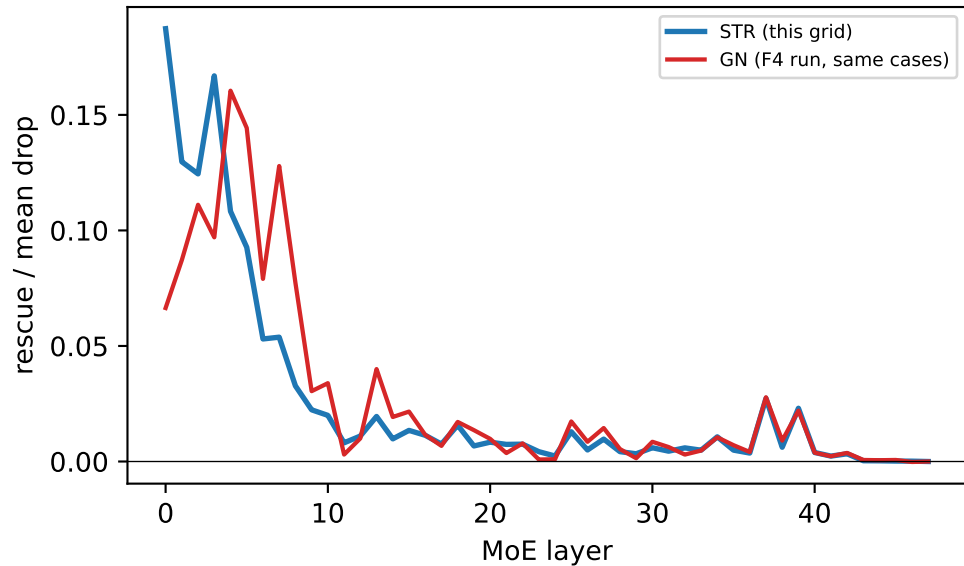
Qwen3-30B-A3B-Base: MoE patch at the last subject token
