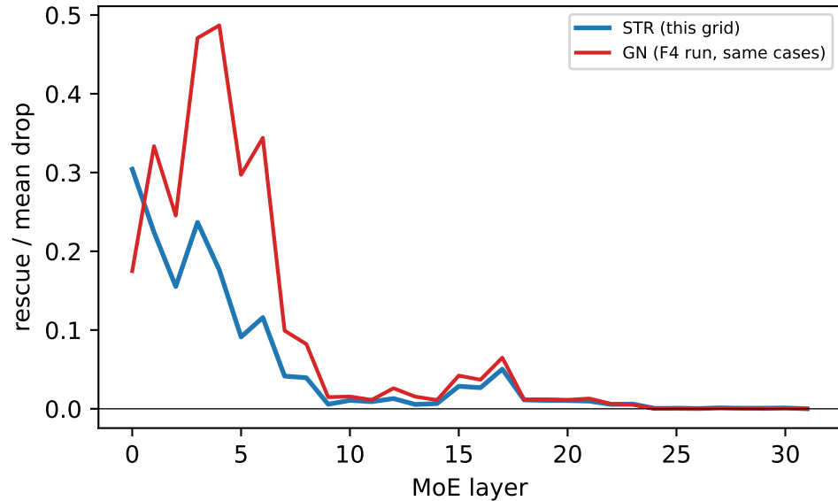
Mixtral-8x7B, BOS: MoE patch at the last subject token
