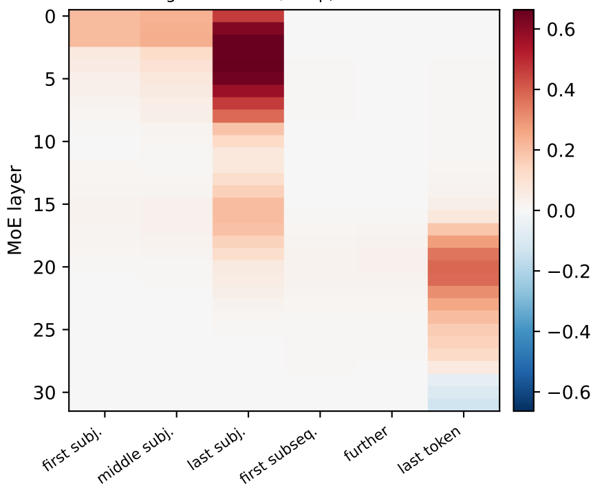
logit difference / drop, window 5
