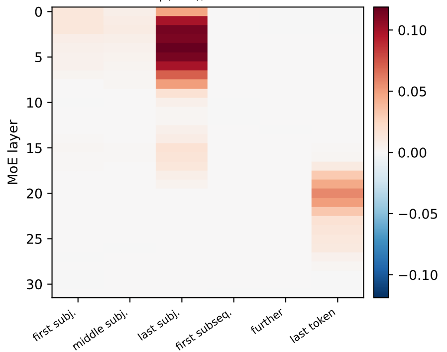
\Delta p(\text{true}) , window 5
