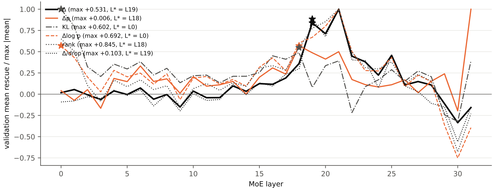
Mixtral-8x7B-v0.1 (no BOS, paper protocol): layer curves under each metric, each scaled by its own maximum (star = discovery ar
