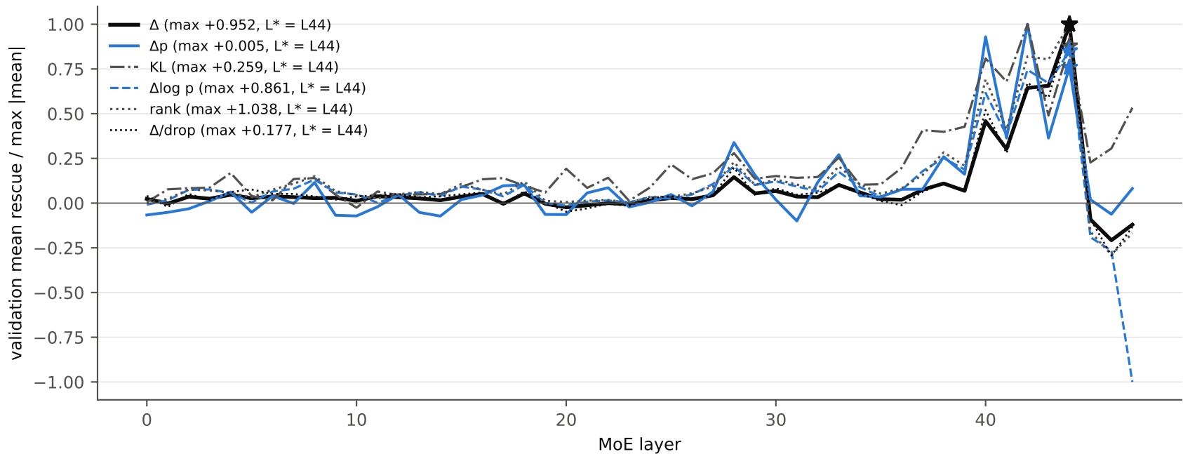
Qwen3-30B-A3B-Base (tokenizer defaults): layer curves under each metric, each scaled by its own maximum (star = discovery arg)
