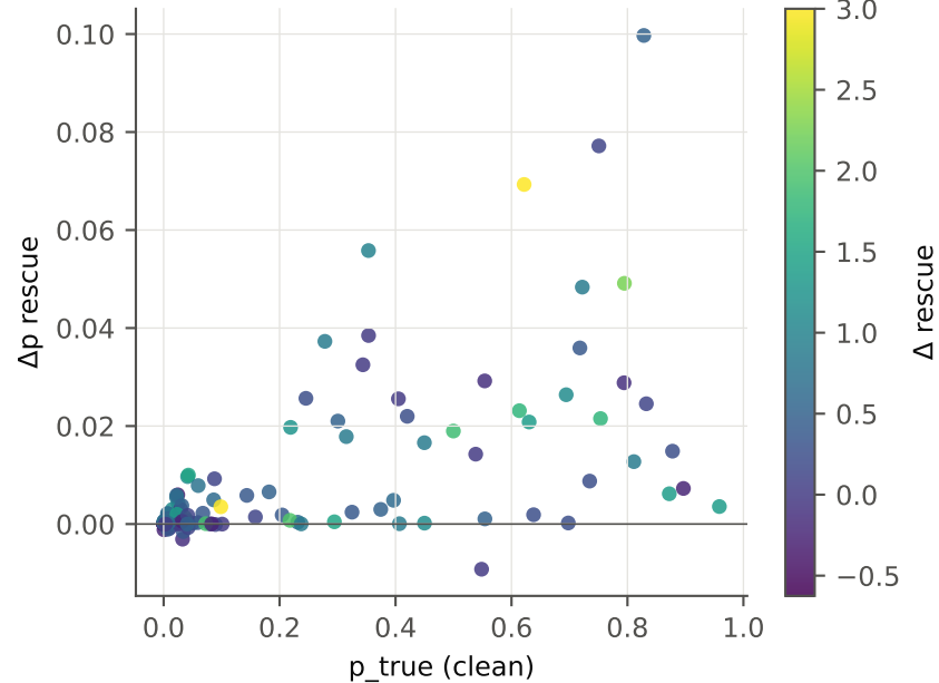
B. \Delta p vs the clean probability (saturation)
