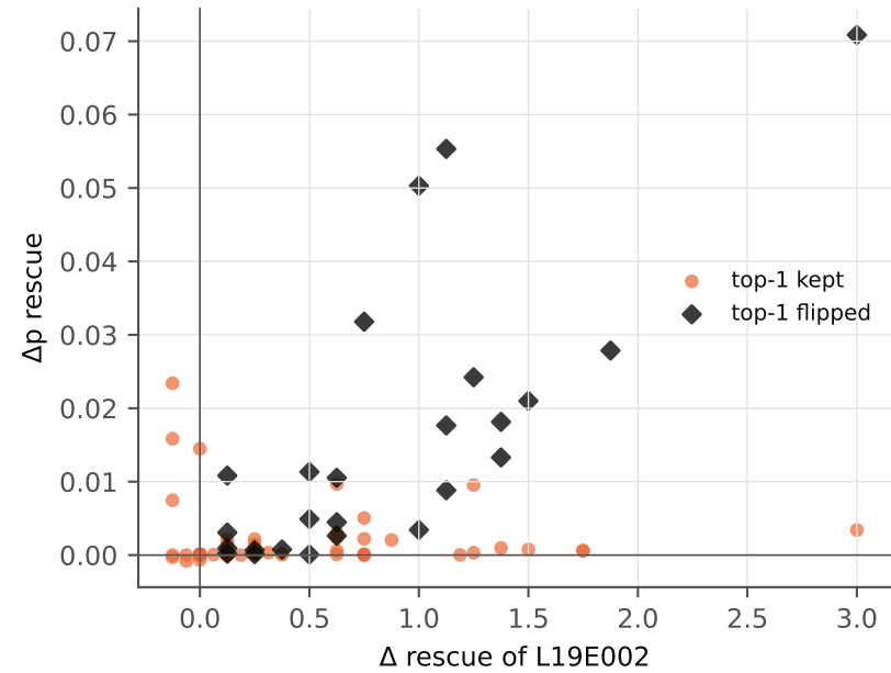
C. selected expert L19E002: \Delta vs \Delta p (active cases)
