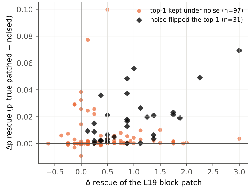
A. block patch at L19: \Delta vs \Delta p per validation case
