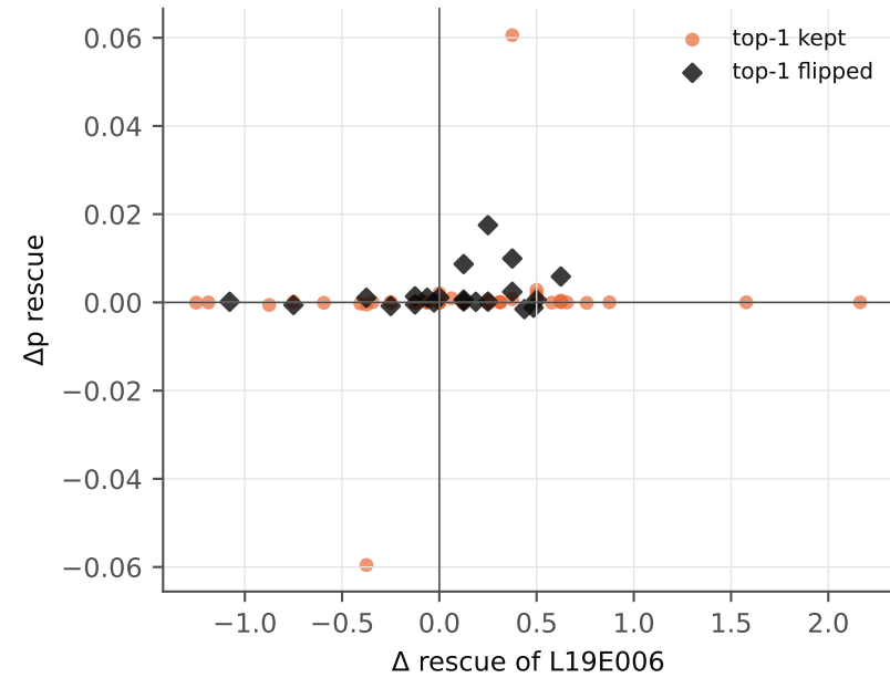
C. selected expert L19E006: \Delta vs \Delta p (active cases)
