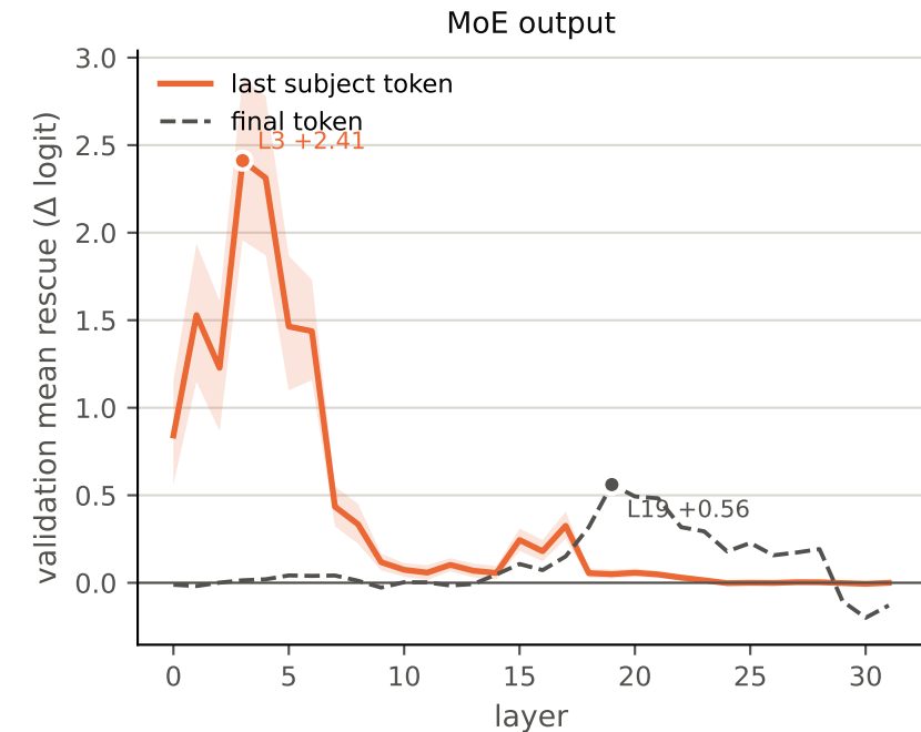
Mixtral-8x7B-v0.1 (BOS, tokenizer default): patch at the last subject token (solid, 95% band) vs the final token (dashed)
