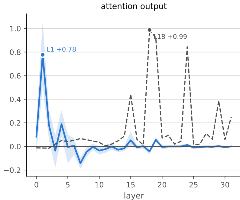
Mixtral-8x7B-v0.1 (BOS, tokenizer default): patch at the last subject token (solid, 95% band) vs the final token (dashed)
