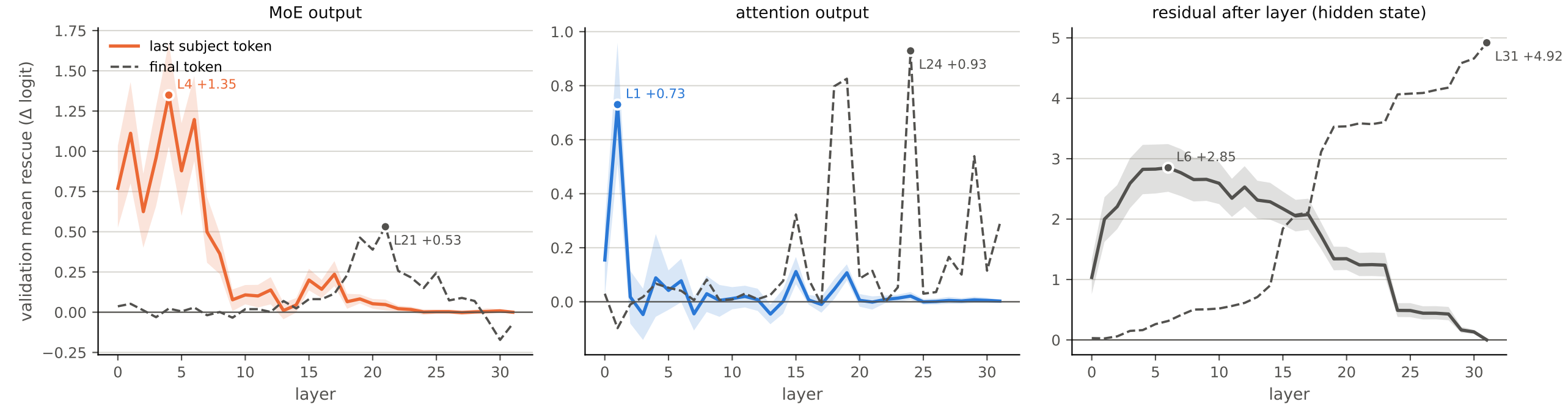
Mixtral-8x7B-v0.1 (no BOS, paper protocol): patch at the last subject token (solid, 95% band) vs the final token (dashed)
