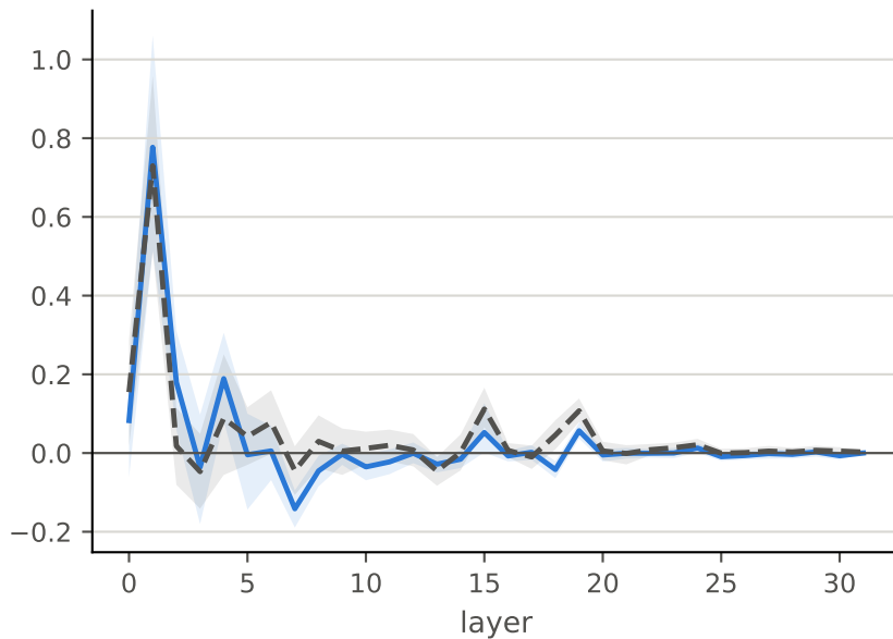
attention output at the last subject token
