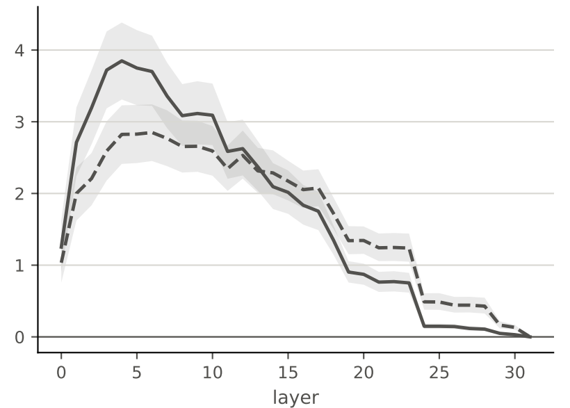
residual after layer (hidden state) at the last subject token
