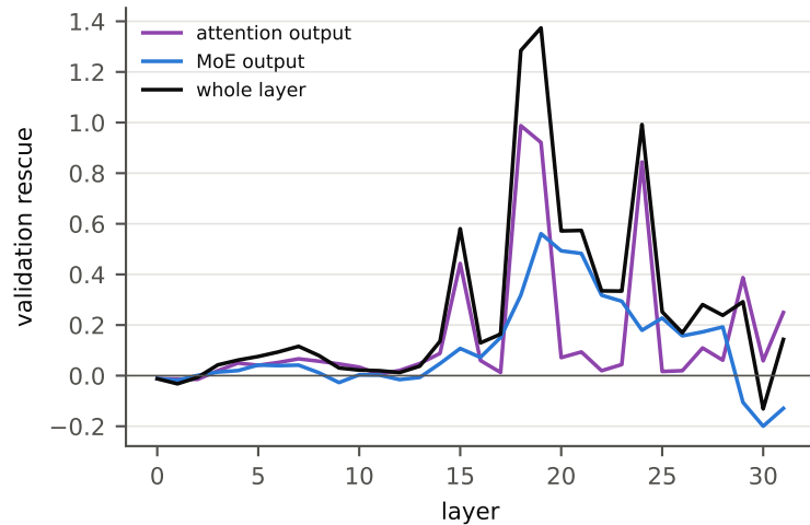
Mixtral-8x7B-v0.1 — default [paper, n=128]
