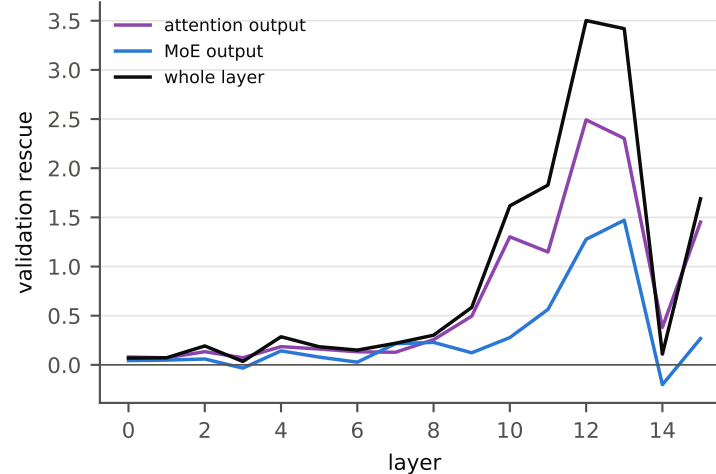
Mixtral-8x7B-Instruct-v0.1 — chat [paper, n=128]
