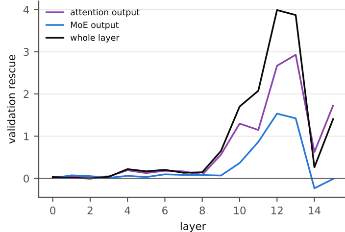
Qwen3-Coder-30B-A3B-Instruct — chat [paper, n=128]
