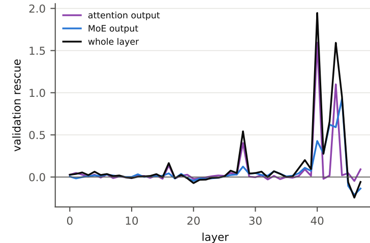
Qwen3-30B-A3B-Base — default [paper, n=128]
