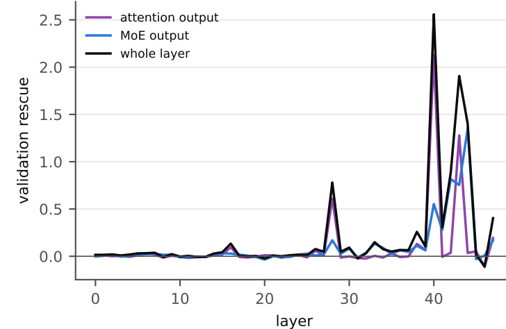
Qwen3-30B-A3B-Base — default [paper, n=128]
