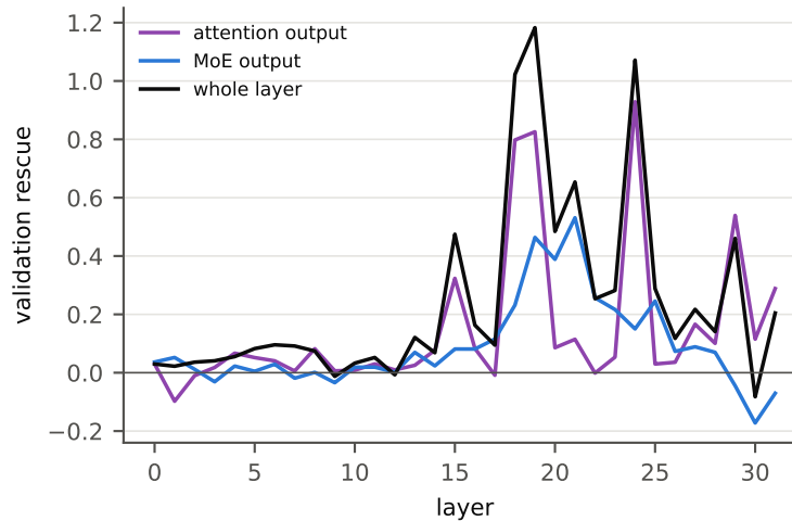
Mixtral-8x7B-v0.1 — nobos [paper, n=128]
