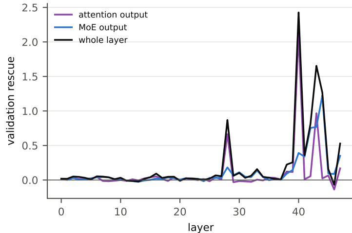
Mixtral-8x7B-v0.1 — default [paper, n=128]
