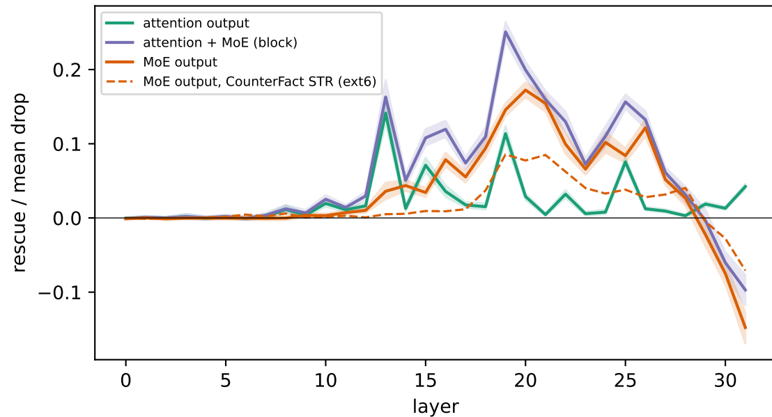
Mixtral-8x7B, BOS: WinoGrande STR, final position (validation, 128 pairs)
