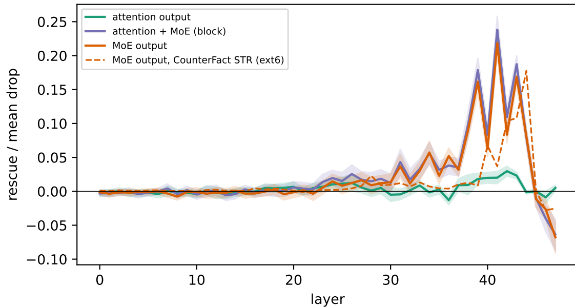
Qwen3-30B-A3B-Base: WinoGrande STR, final position (validation, 128 pairs)
