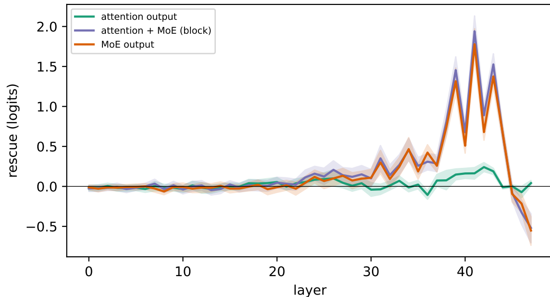
Qwen3-30B-A3B-Base: WinoGrande STR, final position (validation, 128 pairs)
