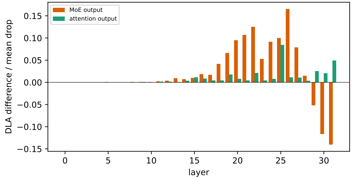
Mixtral-8x7B, BOS: direct logit attribution of the final-position sublayer outputs (clean – corrupted)
