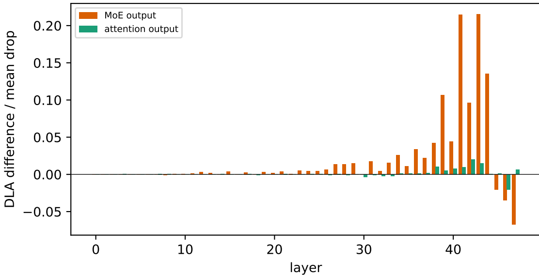
Qwen3-30B-A3B-Base: direct logit attribution of the final-position sublayer outputs (clean – corrupted)
