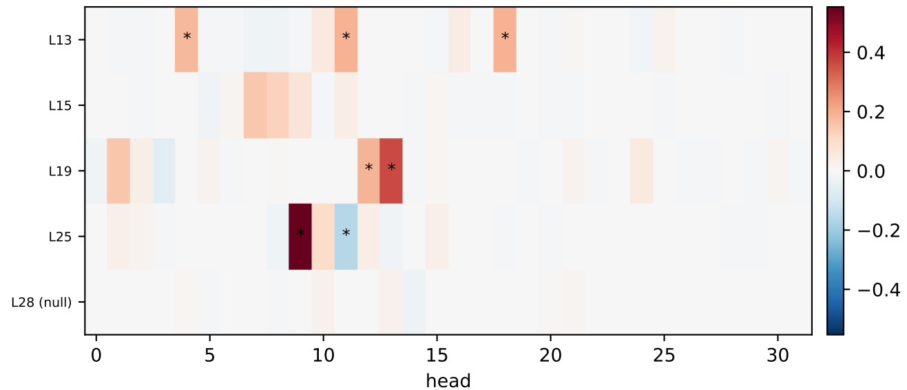
Mixtral-8x7B, BOS: per-head attention patch at the final position (validation rescue, logits)
