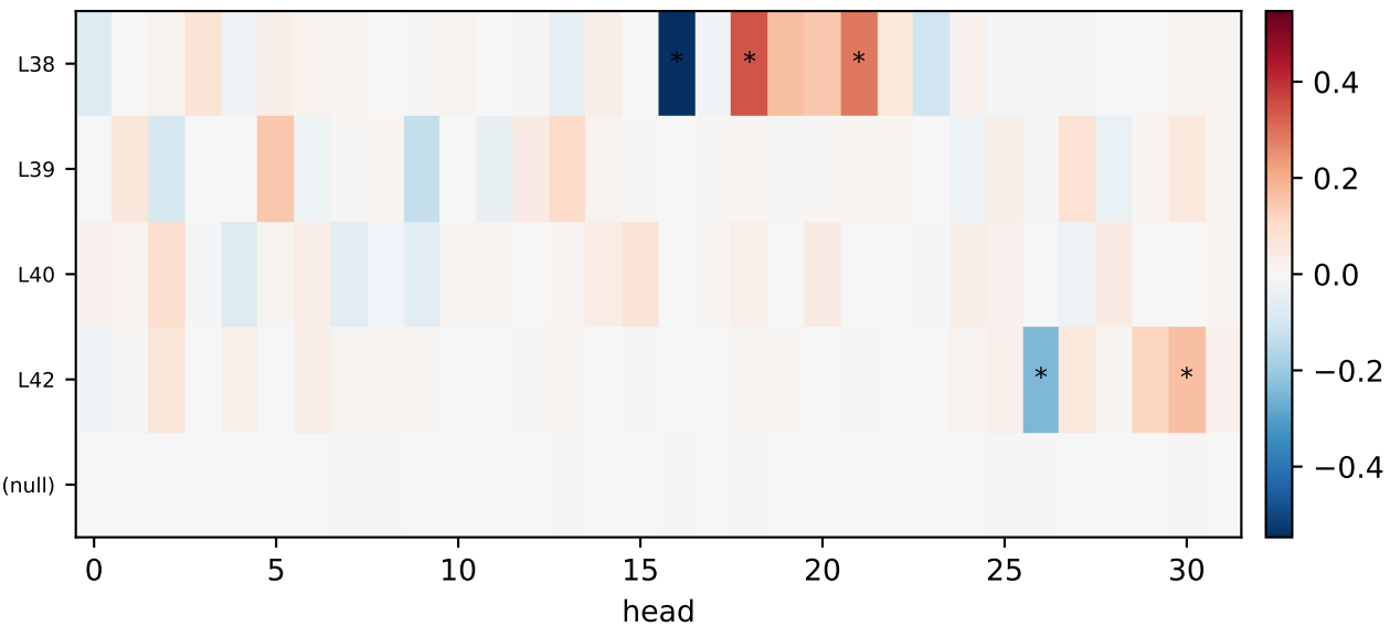
Qwen3-30B-A3B-Base: per-head attention patch at the final position (validation rescue, logits)
