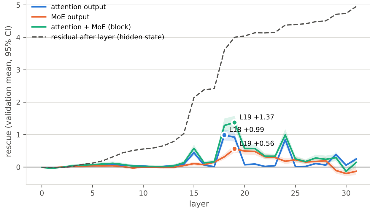
Mixtral-8x7B-v0.1 (BOS, tokenizer default): rescue by patched component
