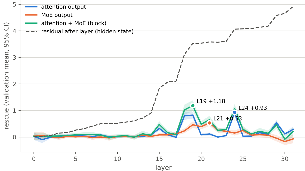
Mixtral-8x7B-v0.1 (no BOS, paper protocol): rescue by patched component
