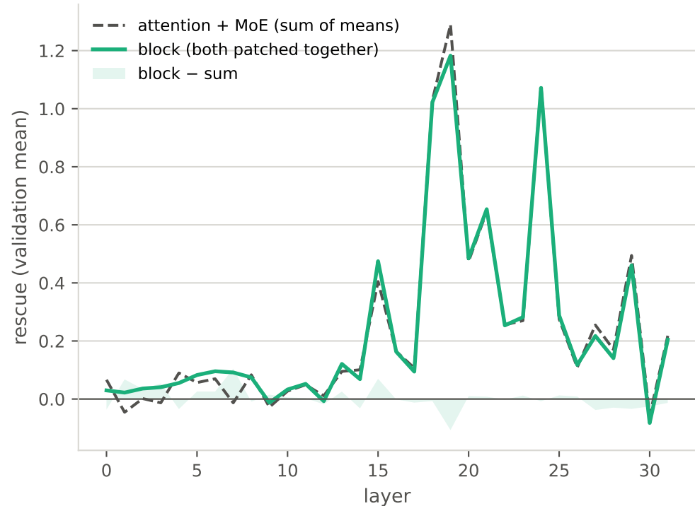
additivity: block vs attention + MoE
