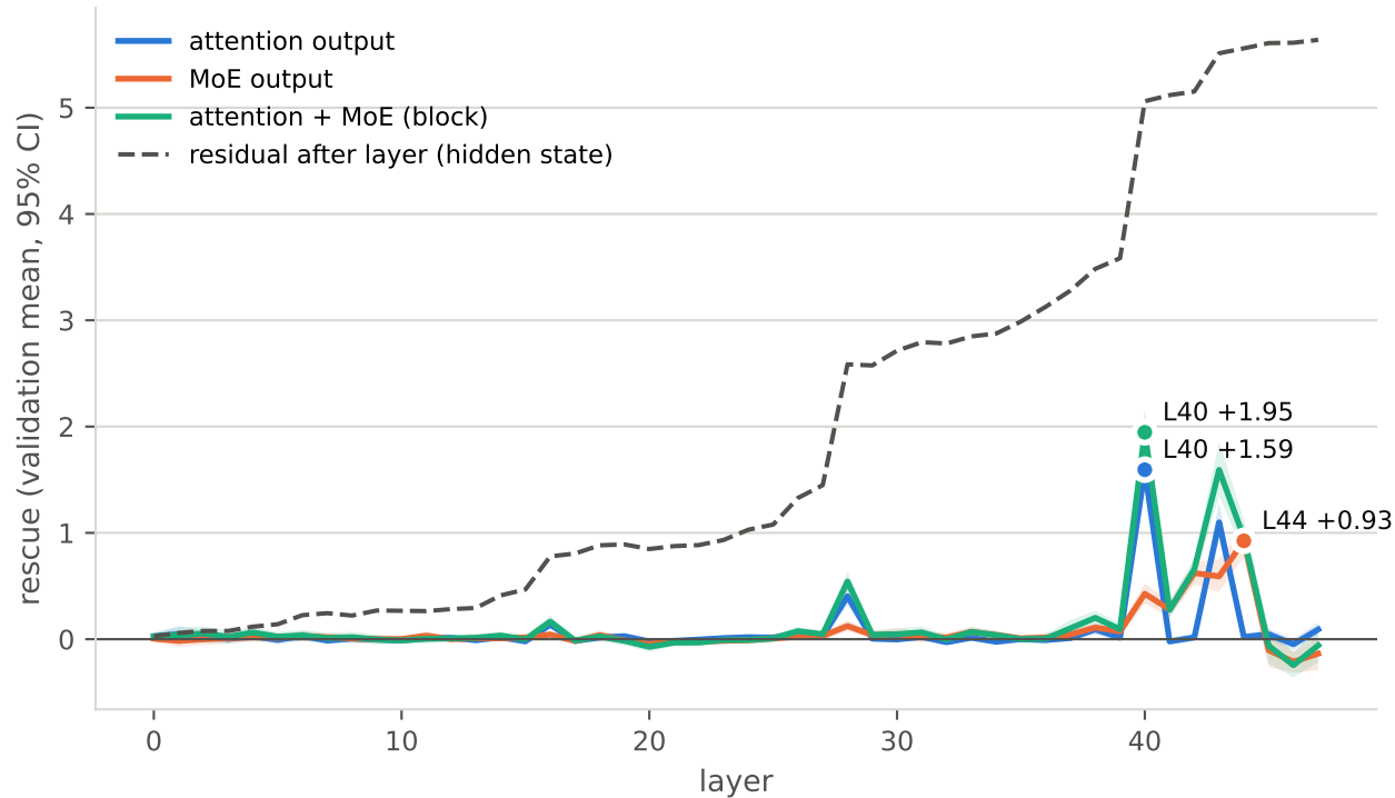
Qwen3-30B-A3B-Base (tokenizer defaults): rescue by patched component
