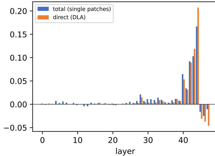
Qwen3-30B-A3B-Base CounterFact
