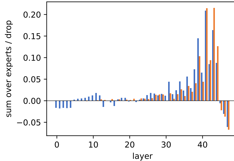
Qwen3-30B-A3B-Base WinoGrande
