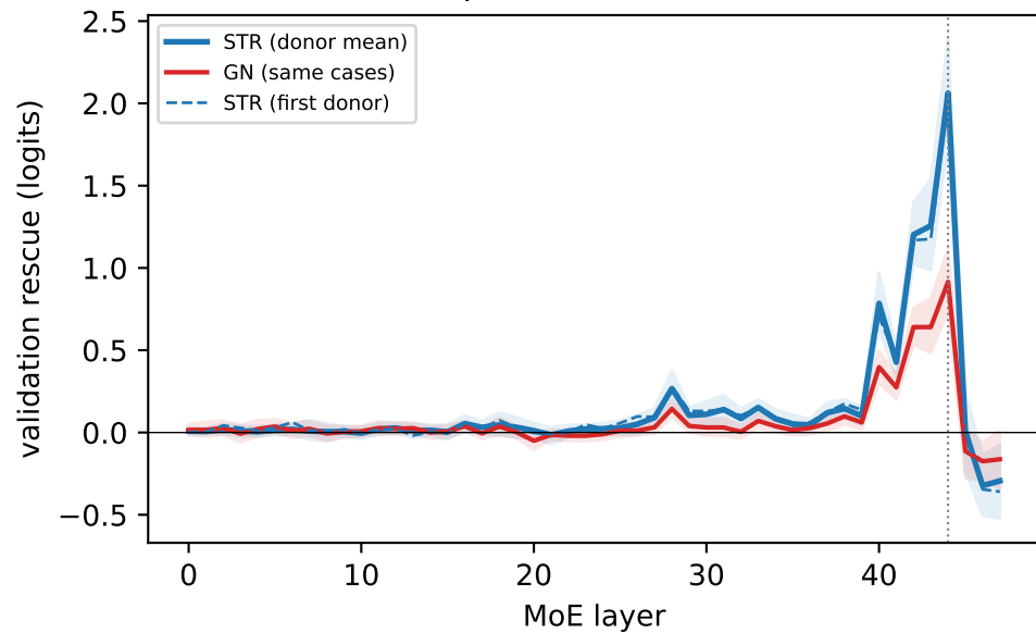
Qwen3-30B-A3B-Base
