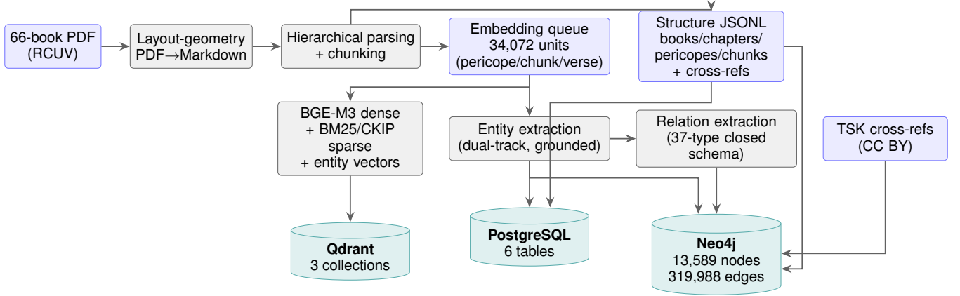
Fig. 1. Offline build pipeline. Every arrow is a materialized JSONL hand-off; the three databases play complementary roles (Section V-A); database counts show the live post-remediation state (July 6, 2026). The embedding queue doubles as the extraction feed — the structural root cause analyzed in Section VIII (mechanism M1).
