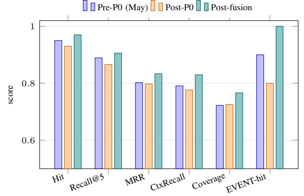
Fig. 4. The three-round shape of the evidence chain: the KG completeness overhaul alone (orange) reads flat-to-negative on a head-entity benchmark; unlocking the ranking layer (teal) recovers and surpasses every indicator.
