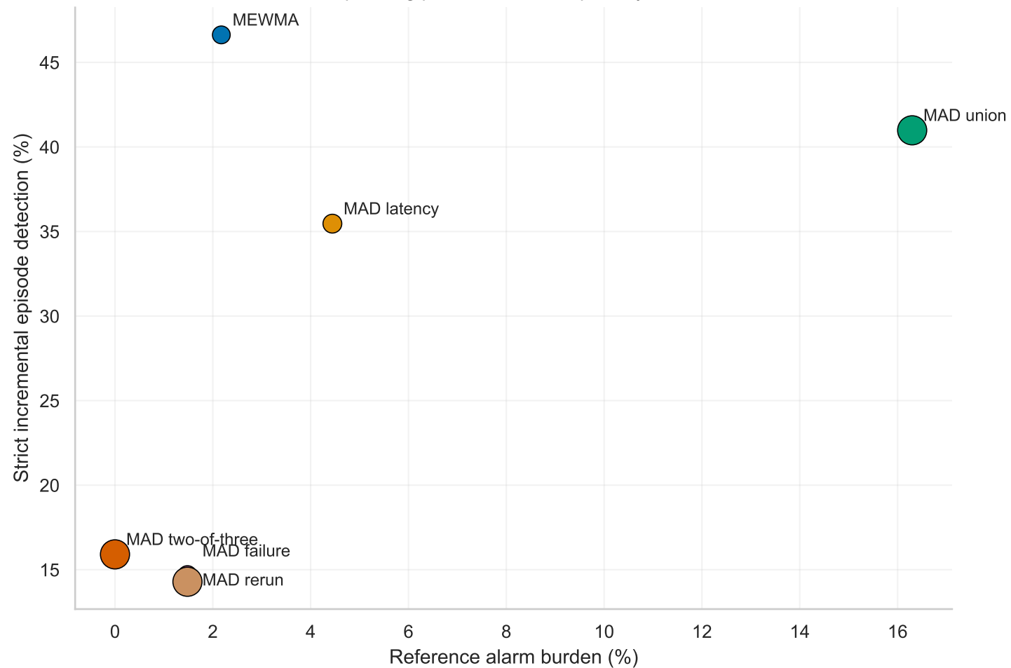
Detector operating profiles under the primary data condition
