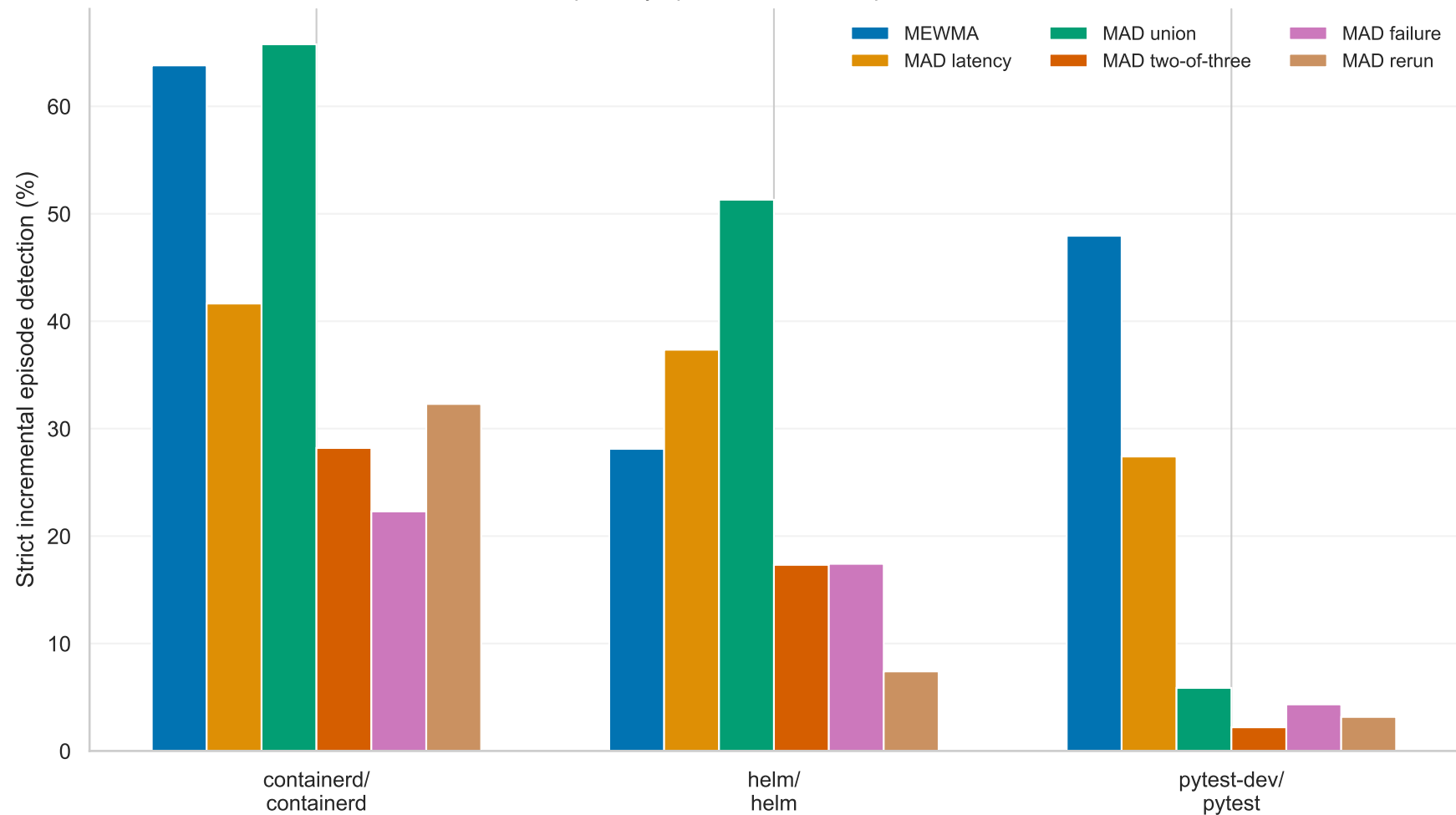
Repository-specific detector responsiveness
