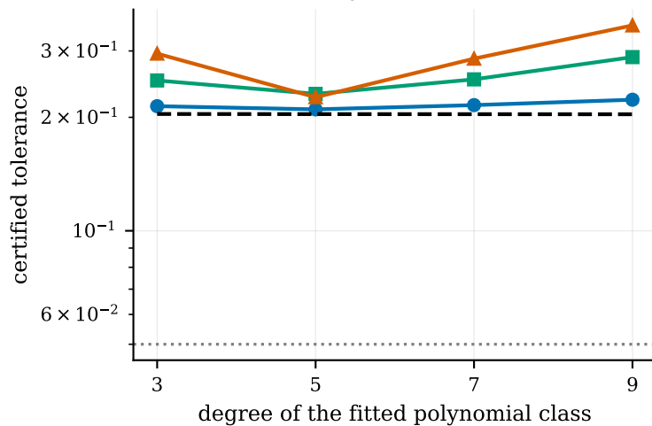
(b) no continuous symmetry (pendulum, not polynomial)
