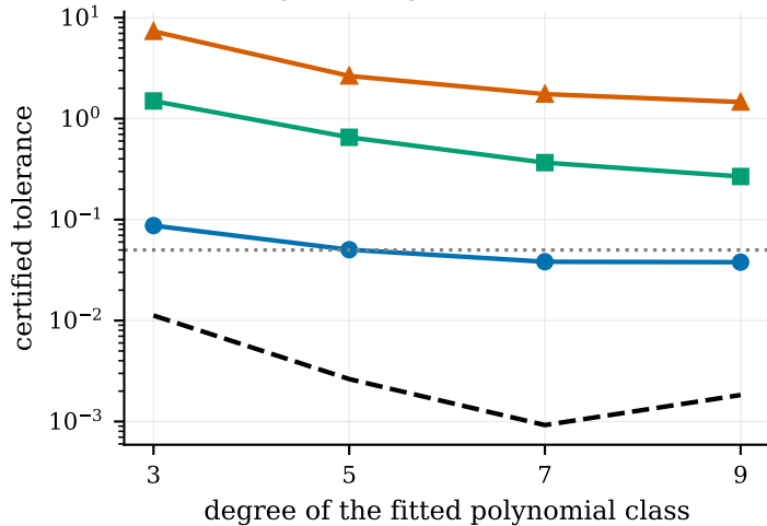
(a) exact rotational symmetry (rot nonpoly, not polynomial)
