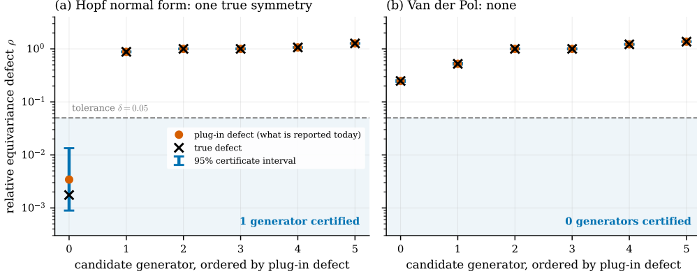
Figure 1: What the procedure outputs, on two systems at N = 3200 and noise level 0.03. Each candidate generator gets an interval for its true defect, valid simultaneously across all six. A generator is certified when its interval lies entirely inside the shaded region below the tolerance. On the Hopf normal form the rotation generator is certified; on Van der Pol nothing is, correctly, and the lower certificate goes further, ruling out at 95% confidence the existence of any generator in the class with defect below 0.14. For the large defects the intervals are narrower than the plotting symbols: the certificate is only wide where the answer is genuinely uncertain.
