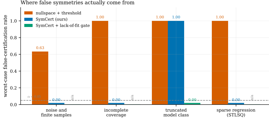
Figure 3: Worst-case false-certification rate under each of the four candidate mechanisms, at tolerance \delta = 0.05 . Noise and finite samples alone are the mildest; incomplete coverage and, above all, the model class are what manufacture symmetry. SYMCERT controls the first two by construction. It does not control the third, because its validity is conditional on the model class containing the truth; a lack-of-fit test detects every truncated class we tried and restores control (green). The fourth group is sparse regression on a weakly symmetry-breaking system: the sparsity threshold deletes the term that breaks the symmetry, and the resulting model is exactly symmetric. Certifying from the unpruned fit gives a rate of zero.
