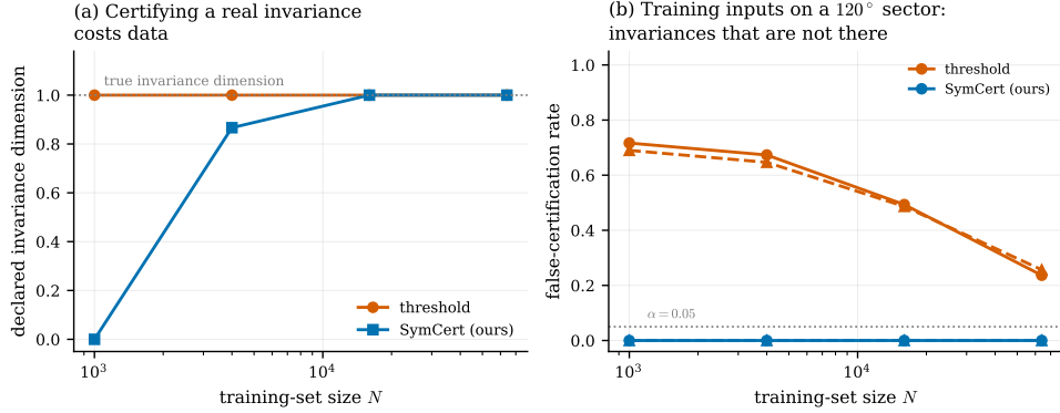
Figure 7: Invariances of a learned model rather than of a dynamical system. (a) With training inputs covering the disc, both rules eventually recover the one-dimensional rotational invariance of the target; certification costs roughly sixteen times more data at this noise level. (b) With training inputs confined to a 120^\circ sector, the fitted model is unconstrained elsewhere, and the threshold rule declares invariances that the target does not have. Solid lines are the rotation-invariant target, dashed the target with no invariance; the two are almost indistinguishable, which is the point, since the threshold rule fails the same way whether or not there is anything to find. SYMCERT declines in both cases.
