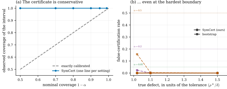
Figure 6: (a) Observed coverage of the certificate interval against its nominal level, one line per setting. The certificate over-covers: the bound treats numerator and denominator separately over the whole confidence ellipsoid. (b) The deliberately hardest case: a system whose true defect sits just above the tolerance, observed at the sample size that puts the median certified bound exactly at the tolerance. SYMCERT (solid) never certifies falsely; a calibration-targeting bootstrap (dashed), which has no finite-sample guarantee, does. Colour marks the nominal level, matching the dotted reference lines.
