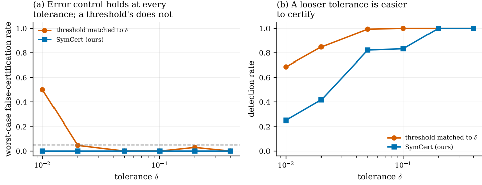
Figure 5: Sweeping the tolerance, on a smaller grid: six systems, two sample sizes, two noise levels. (a) SYMCERT’s worst-case false-certification rate is zero at every tolerance; the threshold rule matched to the same \delta exceeds the nominal level at the tightest one and happens to stay below it at the rest; on the full grid of Table 1 it does not. (b) The tolerance is a real choice rather than a nuisance parameter: it is the approximation the user is willing to accept, and accepting more of it makes symmetry easier to certify, from a detection rate of 0.25 at \delta = 0.01 to 1.00 at \delta = 0.2 .
