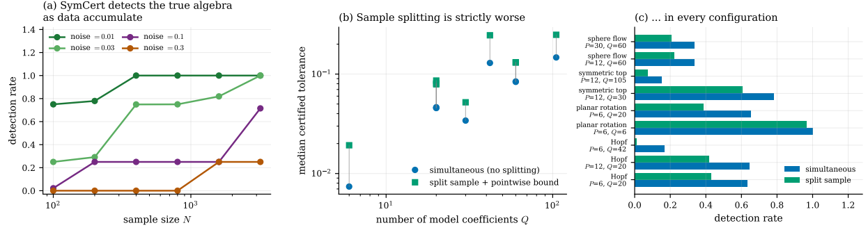
Figure 4: (a) The price of validity is detection power, and it is paid in sample size: at noise level 0.01 SYMCERT recovers the full true algebra in every replication from N = 400 ; at noise level 0.3 it does not, because the data do not support the claim. (b,c) Simultaneity versus sample splitting. Each point in (b) is one model configuration; the simultaneous certificate (blue) is narrower than the split-sample certificate (green) in all nine, by factors of 1.5 to 2.6, and (c) its detection rate is higher in all nine. Splitting protects against a selection effect that simultaneity already removes, and pays for that protection with half the data.
