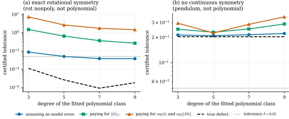
Figure 8: Certifying a system that is not in any polynomial class. Ignoring the approximation error (blue) gives a bound that is not valid; paying for it in supremum norm (orange) is valid but vacuous; paying for it in L^2 against a richer polynomial class (green) is valid and several times tighter, and improves as the fitted class grows, though on the left-hand system it is still above the tolerance at degree 9, so the exact rotational symmetry that is really there cannot be certified honestly at this sample size. The dashed line is the true defect, obtained by Monte-Carlo integration of the analytic bracket; the dotted line is the tolerance \delta = 0.05 .
