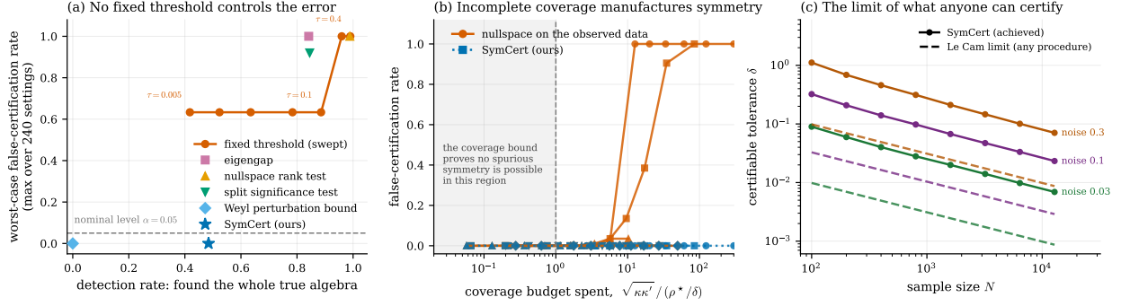
Figure 2: (a) Every method is placed by how often it finds the whole true symmetry algebra (horizontal) against the largest false-certification rate it produces over the 240 settings (vertical). The orange curve traces the fixed-threshold rule as the tolerance is swept from 0.005 to 0.4: no choice of tolerance brings its worst case near the nominal level (dashed). The rank test and the split-sample significance test are valid level-0.05 tests, and are among the worst discovery rules, because failing to reject “this is a symmetry” is read as evidence for it. SYMCERT is at 0; the Weyl perturbation bound is also at 0 but never certifies anything. (b) Shrinking the region the data occupy while keeping the claim about the full domain. The horizontal axis is the extrapolation bound of Proposition 10 divided by the value it must reach before a spurious symmetry is arithmetically possible. In the shaded region the proposition proves no spurious symmetry can occur, and none does in any of the 13 settings there; beyond it the nullspace rule fails on 14 of 37 settings. SYMCERT (blue) is at zero throughout, declining to certify rather than certifying wrongly. (c) The tolerance that can be certified about a truly symmetric system, against the Le Cam limit of Proposition 9 for any procedure with the same error control. Both scale as \sigma/\sqrt{N} ; the gap is a constant factor of 8.1–8.8.
