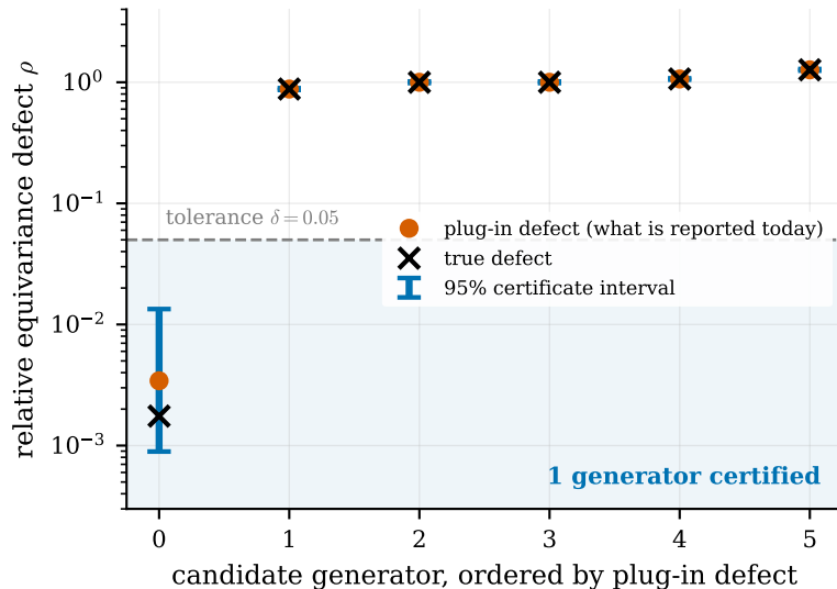
(a) Hopf normal form: one true symmetry
