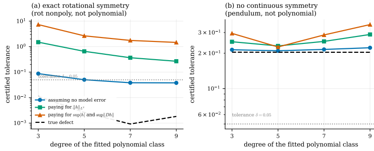
Fig. 8 Certifying a system that is not in any polynomial class. Ignoring the approximation error (blue) gives a bound that is not valid; paying for it in supremum norm (orange) is valid but vacuous; paying for it in L^2 against a richer polynomial class (green) is valid and several times tighter, and improves as the fitted class grows, though on the left-hand system it is still above the tolerance at degree 9, so the exact rotational symmetry that is really there cannot be certified honestly at this sample size. The dashed line is the true defect, obtained by Monte-Carlo integration of the analytic bracket; the dotted line is the tolerance \delta = 0.05 .
