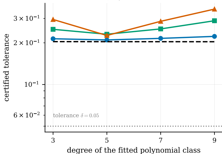
(b) no continuous symmetry (pendulum, not polynomial)
