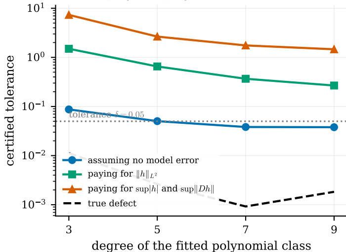
(a) exact rotational symmetry (rot nonpoly, not polynomial)
