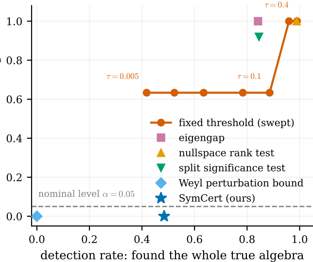
(a) No fixed threshold controls the error
