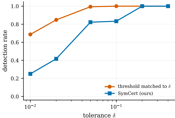
(b) A looser tolerance is easier to certify
