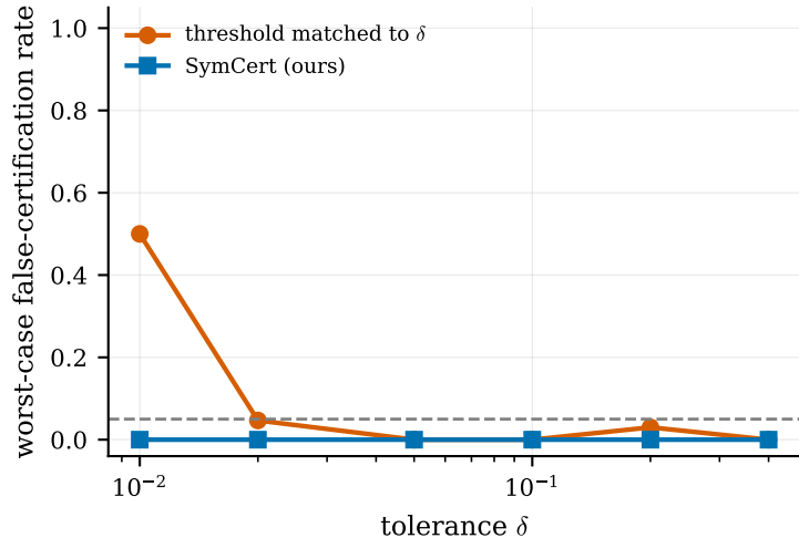
(a) Error control holds at every tolerance; a threshold's does not
