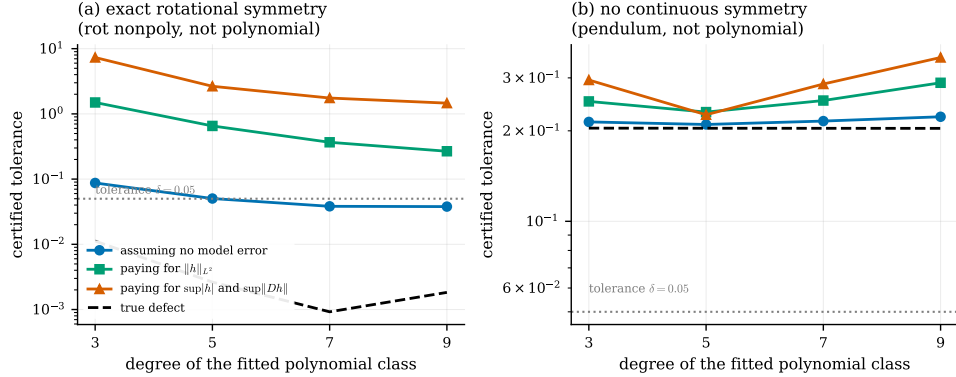
Figure 8: Certifying a system that is not in any polynomial class. Ignoring the approximation error (blue) gives a bound that is not valid; paying for it in supremum norm (orange) is valid but can be vacuous; paying for it in L^2 against a richer polynomial class (green) is valid and informative, and improves as the fitted class grows. The dashed line is the true defect, obtained by Monte-Carlo integration of the analytic bracket.
