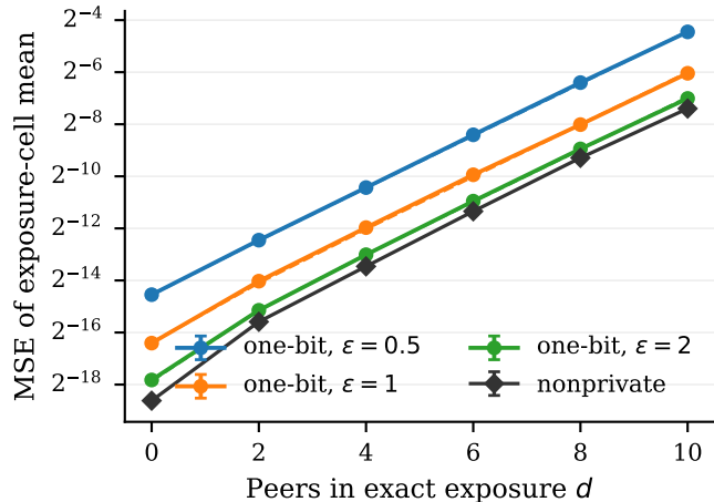
Raw risk grows as 2^d
