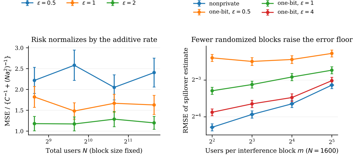
Figure 2: Diagnostics for the two risk components. Left: observed one-bit MSE divided by C^{-1} + (Na_\epsilon^2)^{-1} stays within a budget-specific constant as N and C grow with m = 8 . Right: at fixed N , increasing m reduces the number of first-stage randomized blocks and raises the nonprivate floor, while tight-privacy error is comparatively flat.
