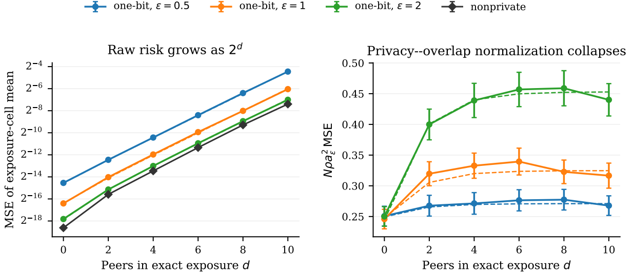
Figure 3: Privacy multiplies exact-exposure rarity. An exact assignment pattern among d peers has probability \rho = 2^{-d} . Left: HT mean squared error grows geometrically; dashed curves are exact finite- N moment calculations, not fits. Right: the normalized quantity N\rho a_\epsilon^2 \text{MSE} follows those calculations and is nearly constant in d after the dense-cell edge case. Policy-marginal effects avoid selecting this rare cell.
