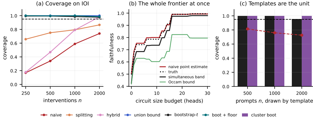
Figure 3: GPT-2 small, IOI. (a) Coverage of each bound at the selected circuit as the number of interventions grows. The naive interval does not improve with n — more data makes the search sharper as fast as it makes the estimate sharper. (b) The size/faithfulness frontier. For every size budget on the horizontal axis, the best-scoring circuit of at most that size is selected and its faithfulness reported. The naive curve (red) lies above the truth (dotted) at every budget; the simultaneous band (black) lies below it at every budget jointly , with probability 0.98. One band certifies the entire reported curve, not one point on it. (c) When prompts are drawn template-by-template — the honest model of how the evaluation set was produced — a bound that treats prompts as independent under-covers badly, and the cluster bootstrap restores validity.
