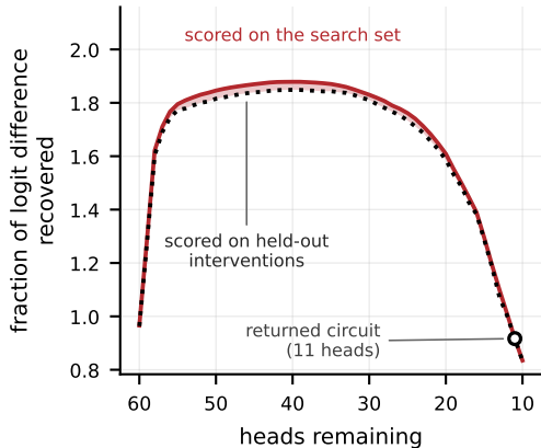
(a) A pruner overfits its own data
