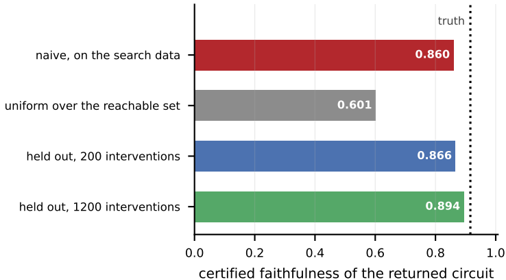
(b) What survives an adaptive search
