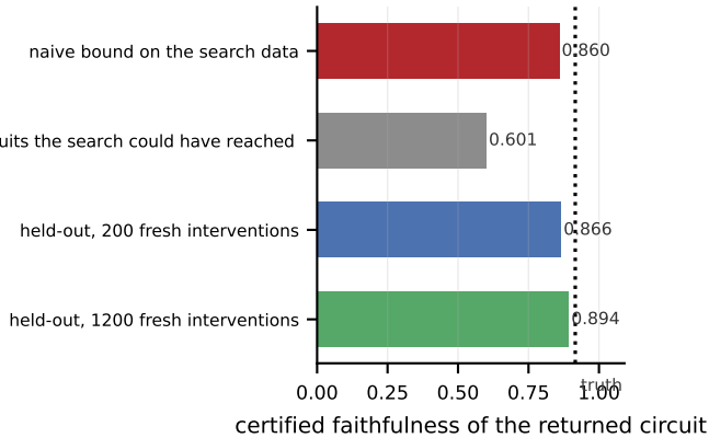
(b) What survives an adaptive search
