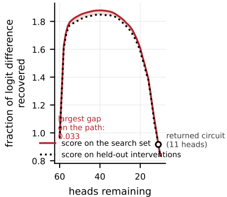
(a) A pruner overfits its own data
