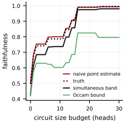
(b) The whole frontier at once
