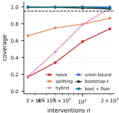
(a) Coverage on IOI
