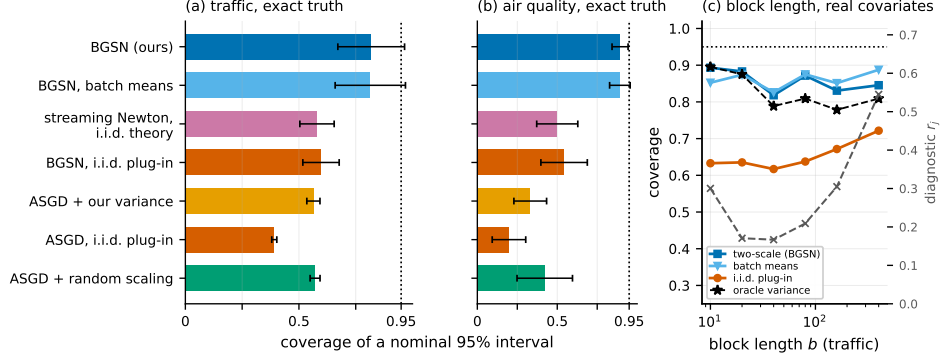
Figure 3: Two real hourly streams. (a, b) Coverage of nominal 95% intervals under Protocol A (real covariates, synthetic autoregressive errors, exact target and exact conditional long-run covariance). The air-quality stream’s median estimated variance inflation is 9.9, so dependence-blind intervals fail badly there. (c) Coverage (left axis) against block length b (horizontal, log scale) on the traffic stream, with the free block-adequacy diagnostic r_j = |u_j^\top (\hat{S}^{\text{FT}} - \hat{S}^{\text{BM}}) u_j| / (u_j^\top \hat{S}^{\text{BM}} u_j) — an estimate of the relative block-length bias of plain batch means, defined where it is first used in Section 5 — on the right axis. Three things to read. Our coverage is flat in b over a fortyfold range and stays within a few hundredths of the infeasible oracle-variance curve throughout, so the shortfall from 0.95 on an 8,000-observation segment is the point estimate and not the covariance. The dependence-blind curve sits far below at every b and does not close. And r_j is U-shaped, lowest near b = 20 –40: it rises for small b , where plain batch means are biased, and again for large b , where too few blocks remain to estimate anything stably — which is what makes it a usable guide to the block length, though not a calibration guarantee.
