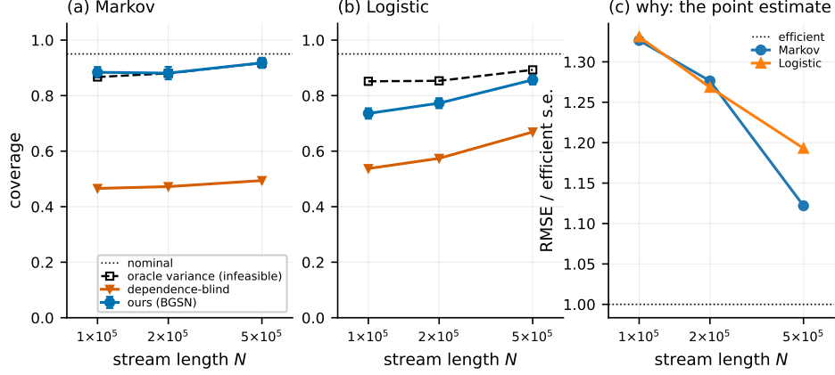
Figure 4: Separating “the variance estimate is wrong” from “the central limit theorem has not taken hold” on the two designs whose point estimate has not converged at the sample sizes of Table 1. (a) The regime-switching design, whose covariate chain has an integrated autocorrelation time of about 66 observations. (b) The dependent-logistic design, where instead the curvature weight \alpha = \sigma'(x^\top \theta) is largest at the \theta_0 the warm-up evaluates it at. In both, the infeasible curve uses the exact H^{-1}SH^{-1} at the same iterate, so the vertical distance between it and ours is everything our covariance estimator is responsible for: that distance is at most 0.017 on the Markov design and falls from 0.116 to 0.036 on the logistic one. Ours and the infeasible curve rise towards nominal together; the dependence-blind curve does not. (c) Why both left panels start low: the root-mean-square error of the point estimate, divided by the efficient standard error, is still above one, so \sqrt{N}(\theta_T - \theta^*) is not yet close to its limit and no choice of variance can give nominal coverage.
