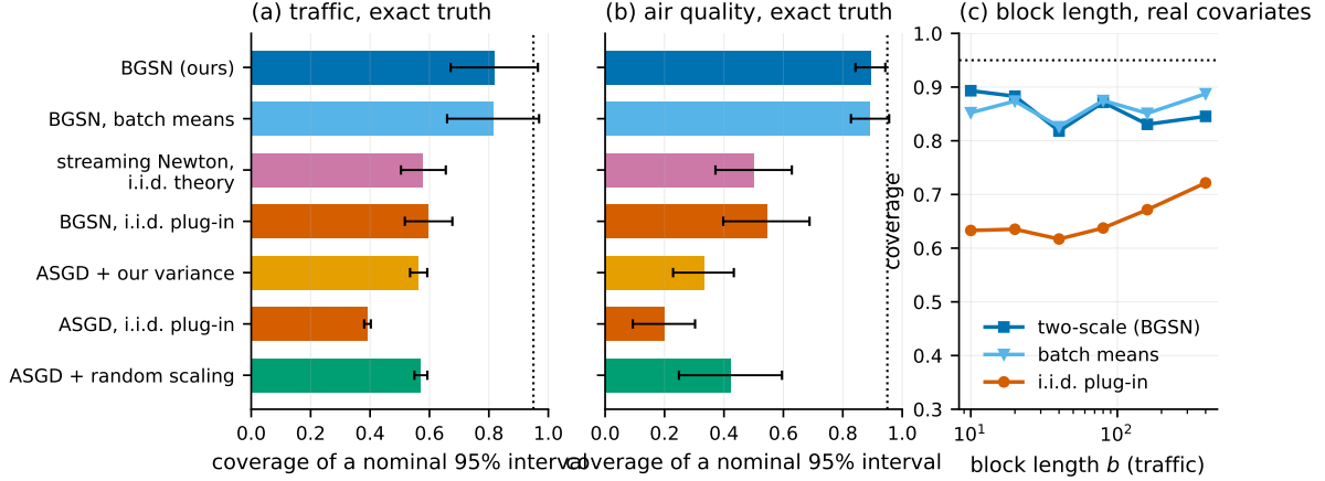
Figure 7: Two real hourly streams. (a, b) Coverage of nominal 95% intervals under Protocol A (real covariates, synthetic autoregressive errors, exact target and exact conditional long-run covariance). The air-quality stream’s median estimated variance inflation is 9.9, so dependence-blind intervals fail badly there. (c) Coverage (vertical) against block length b (horizontal, log scale) on the traffic stream, with the free block-adequacy diagnostic r_j = |u_j^\top (\hat{S}^{\text{FT}} - \hat{S}^{\text{BM}}) u_j| / (u_j^\top \hat{S}^{\text{BM}} u_j) — an estimate of the relative block-length bias of plain batch means, defined where it is first used in Section 5 — overlaid. Coverage improves with b and r_j moves with it; the diagnostic tells you whether b is too small, and it is not a calibration guarantee.
