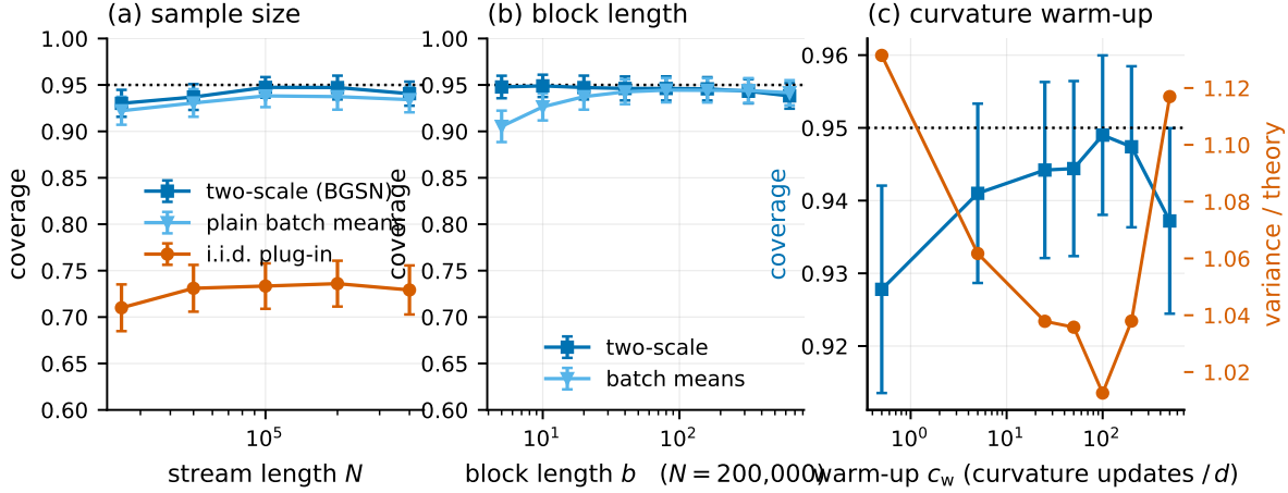
Figure 6: Ablations. (a) Coverage converges to nominal in N for the two-scale variance; the dependence-blind interval converges to 0.749, the value predicted by Proposition 8. (b) Coverage is flat in the block length for the two-scale variance and degrades at both ends for plain batch means. (c) The curvature warm-up is required: without it the 1/t schedule leaves a slowly decaying error that destroys coverage even though the variance estimate is accurate.
