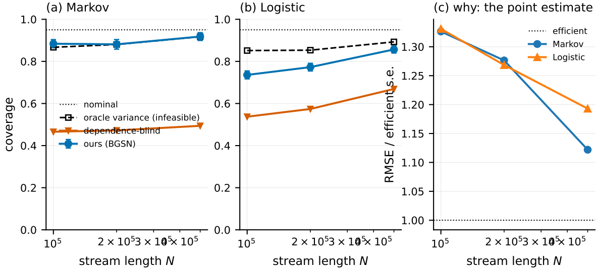
Figure 8: Separating “the variance estimate is wrong” from “the central limit theorem has not taken hold” on the regime-switching design, whose covariate chain has an integrated autocorrelation time of about 66 observations. (a) Coverage of nominal 95% intervals against N . The infeasible curve uses the exact H^{-1}SH^{-1} at the same iterate, so the vertical distance between it and ours is everything our covariance estimator is responsible for; the largest such distance over the sweep is 0.116. Both rise towards nominal; the dependence-blind curve does not. (b) The reason the left panel starts low: the root-mean-square error of the point estimate, divided by the efficient standard error, is still above one at small N , so \sqrt{N}(\theta_T - \theta^*) is not yet close to its limit and no choice of variance can give nominal coverage. (c) why: the point estimate
