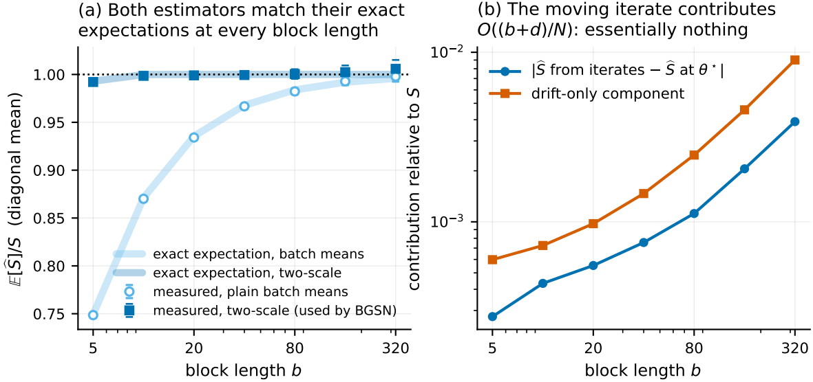
Figure D.1: The long-run covariance estimator, and why the moving iterate does not spoil it. (a) Measured \mathbb{E}[\hat{S}]/S against block length: plain batch means follow the closed-form bias 1 - \Delta/(bS) (no fitted constants), while the two-scale form is unbiased at every b , as Theorem 9 predicts under geometric mixing. (b) The algorithm’s block gradients decomposed exactly into the score at \theta^* and the drift \hat{H}_t(\theta_{t-1} - \theta^*) . The drift’s contribution to \hat{S} is 0.1% of S at b = 20 and 0.9% at b = 320 , growing like (b + d)/N as Theorem 9 predicts, and the estimator built from the algorithm’s iterates is indistinguishable from the one built at \theta^* . This is why our block length need only grow like \log N rather than like a power of N (Remark 1).
