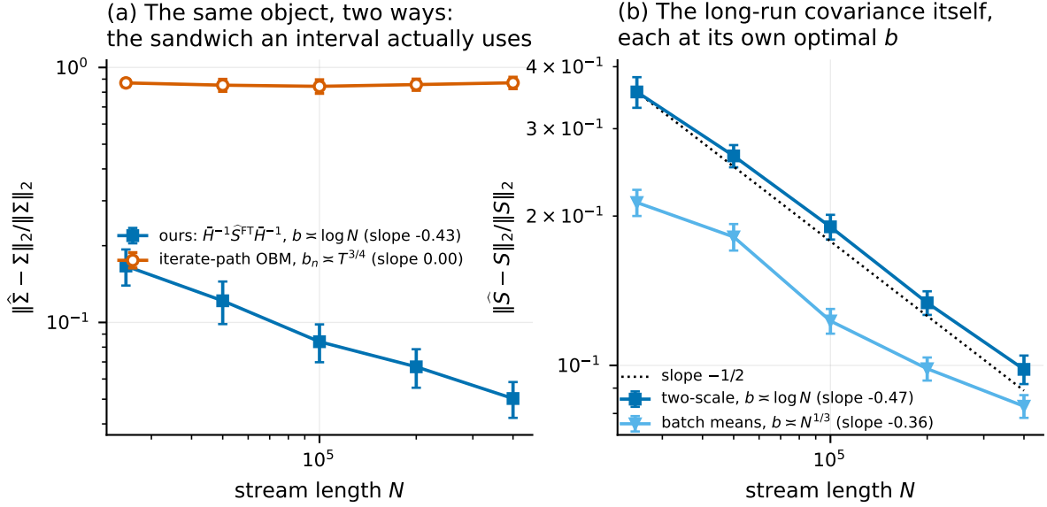
Figure S1: The rate claim, measured, on the object an interval actually uses. Both axes logarithmic; error bars are \pm 1.96 Monte Carlo standard errors; fitted slopes in the legends. (a) Relative operator-norm error in estimating the whole sandwich \Sigma = H^{-1}SH^{-1} . Ours is \bar{H}^{-1}\hat{S}^{\text{FT}}\bar{H}^{-1} at b \asymp \log N ; the comparator is overlapping batch means on the iterate path at the block length b_n \asymp T^{3/4} that analysis requires (Appendix C.3 gives the form), which uses no gradients and no curvature estimate. Same target, so the comparison is meaningful; but read the levels, not the slopes. The iterate-path curve is flat here, and its published N^{-1/8} rate is too slow for our range to resolve, so its fitted slope says nothing about it. What the panel shows is that over the sample sizes we can reach, one estimator is accurate and the other is not. (b) Error in estimating S alone, each estimator at its own optimal block length: the two-scale form at b \asymp \log N against the -1/2 of Theorem 9(iv), plain batch means at b \asymp N^{1/3} against -1/3 .
