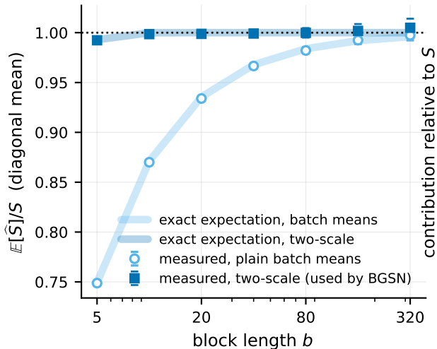
(a) Both estimators match their exact expectations at every block length
