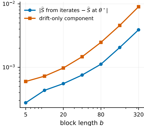
(b) The moving iterate contributes O((b+d)/N) : essentially nothing
