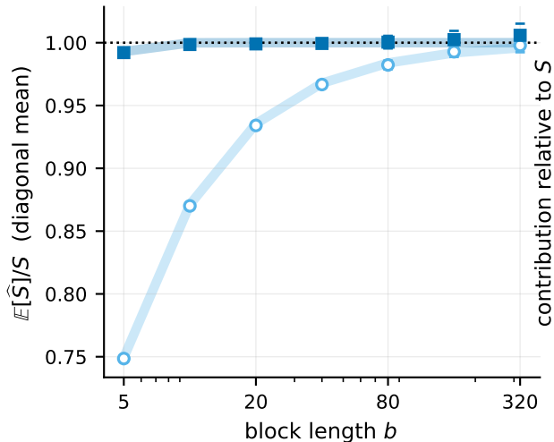
(a) Both estimators match their exact expectations at every block length
