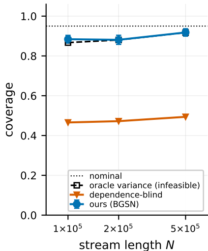
(a) Markov
