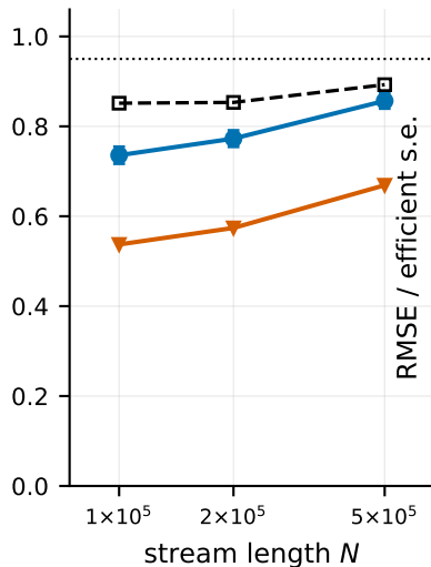
(b) Logistic
