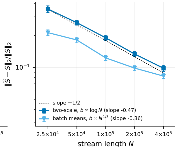
(b) The long-run covariance itself, each at its own optimal b
