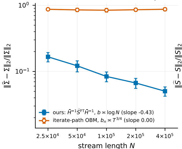
(a) The same object, two ways: the sandwich an interval actually uses
