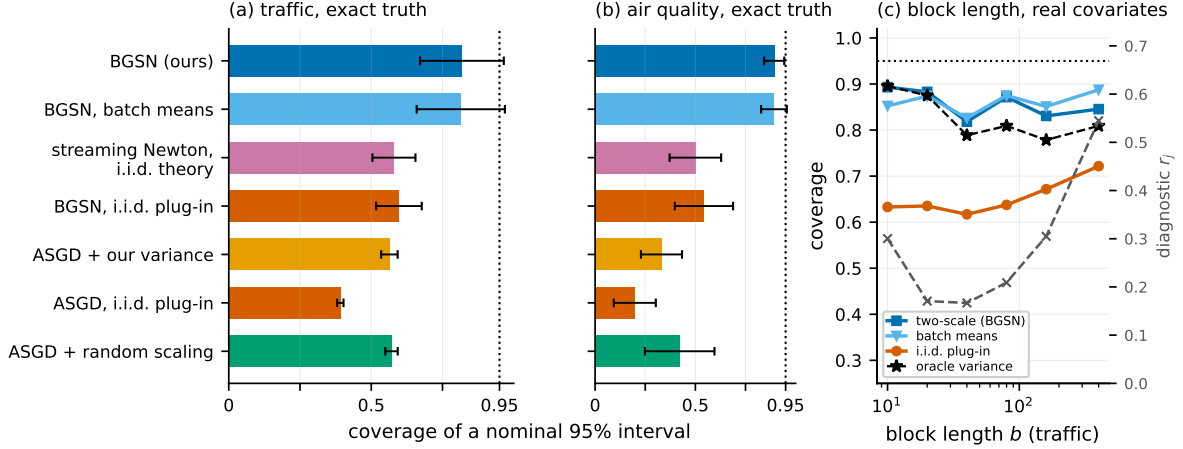
Figure 2: Two real hourly streams. (a, b) Coverage of nominal 95% intervals under Protocol A (real covariates, synthetic autoregressive errors, exact target and exact conditional long-run covariance). The air-quality stream’s median estimated variance inflation is 9.9, so dependence-blind intervals fail badly there. (c) Coverage (left axis) against block length b (horizontal, log scale) on the traffic stream, with the free block-adequacy diagnostic r_j = |u_j^\top (\hat{S}^{\text{FT}} - \hat{S}^{\text{BM}}) u_j| / (u_j^\top \hat{S}^{\text{BM}} u_j) — an estimate of the relative block-length bias of plain batch means, defined where it is first used in Section 5 — on the right axis. Three things to read. Our coverage is flat in b over a fortyfold range and stays within a few hundredths of the infeasible oracle-variance curve throughout, so the shortfall from 0.95 on an 8,000-observation segment is the point estimate and not the covariance. The dependence-blind curve sits far below at every b and does not close. And r_j is U-shaped, lowest near b = 20 –40: it rises for small b , where plain batch means are biased, and again for large b , where too few blocks remain to estimate anything stably — which is what makes it a usable guide to the block length, though not a calibration guarantee.
