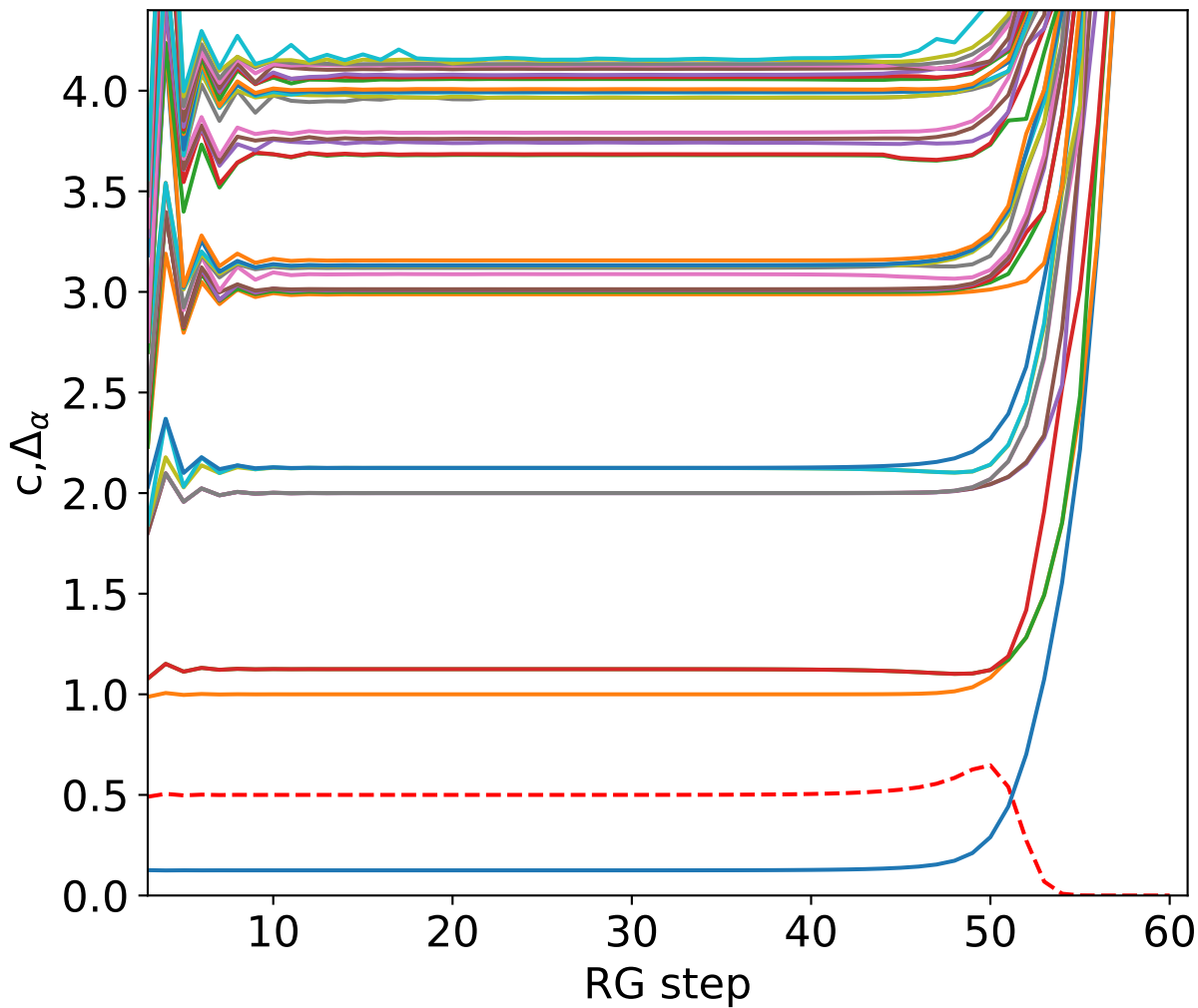
Ising CFT data by NNR-TNR ( \chi = 32 )
