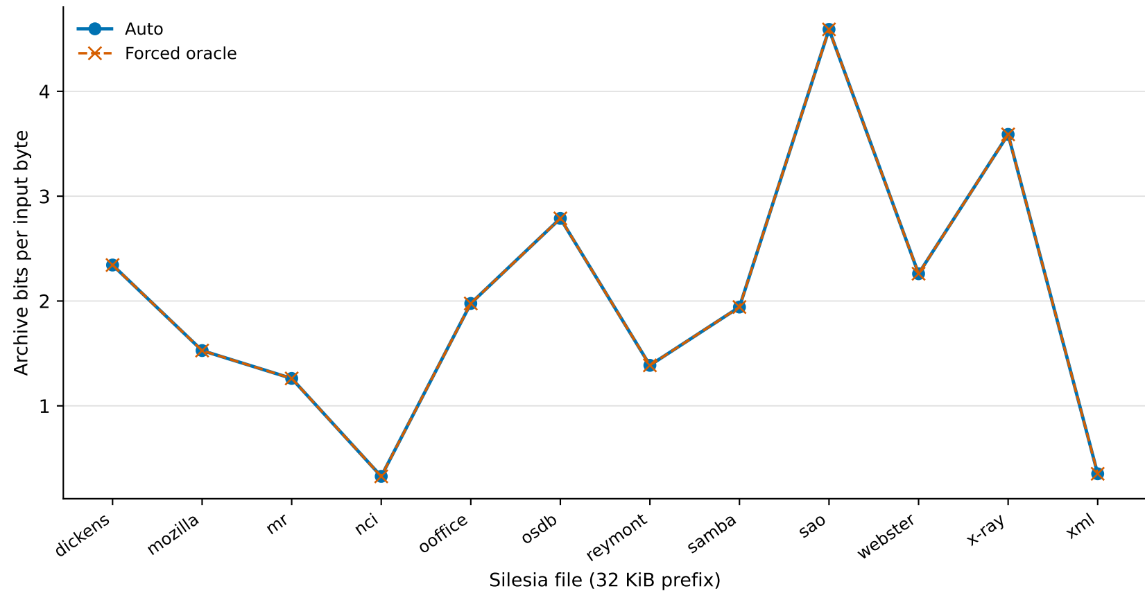
Auto matches the complete forced-mode oracle on every case
