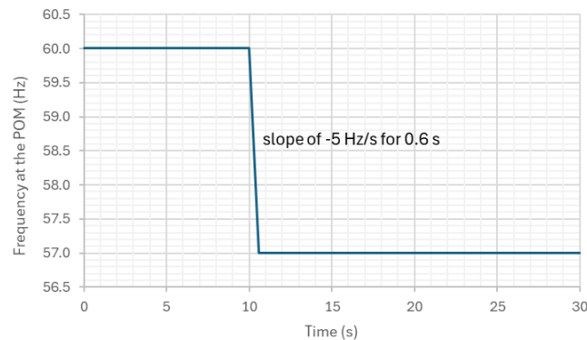
Figure 128: Low frequency profile at the POM for the LFRT tests.
