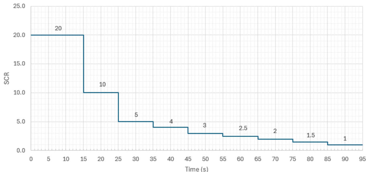
Figure 1410 : Example of short circuit ratio profile of the grid for SCR tests.
