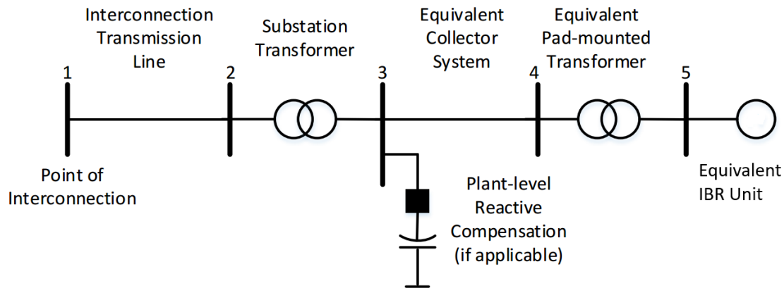
Figure 62. Simplified single-line diagram of an aggregated IBR plant.
