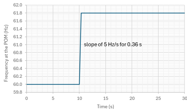
Figure 117: High frequency profile at the POM for the HFRT tests.
