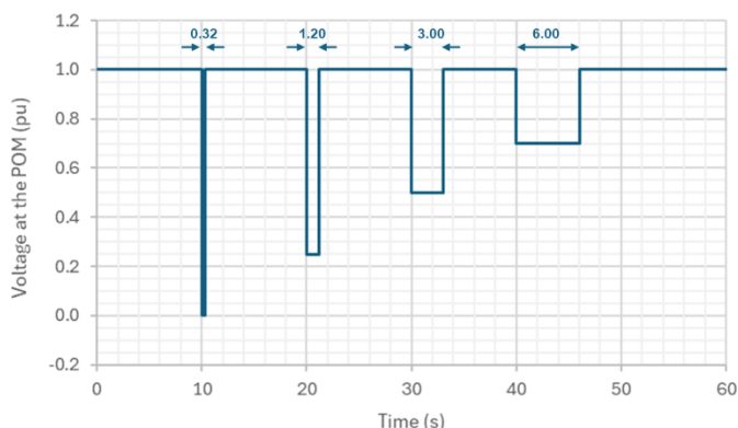
Figure 106 : Low voltage profile at the POM for the LVRT tests.
