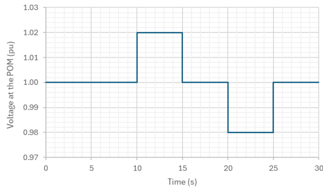
Figure 73: Voltage profile at the POM for the SVD tests.
