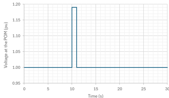
Figure 95: High voltage profile at the POM for the HVRT tests.
