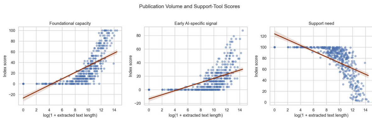
Figure 6. Publication volume and support-tool scores.
